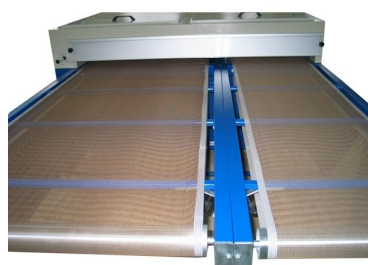
Possibility to equiped dryer with 2 belt systems (2º belt can be the return from garment to operator)
