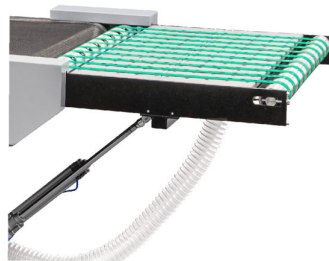
Equipped with 2x high performance UV lamps "CROSS OVER" equipped with pneumatic cylinders to control UP/DOWN
