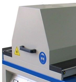
UV Lamp housing 100% closed equipped with crystal quartz glass so no heat is transmit to drying object
