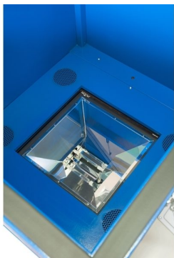
Light source metal/halogen equipped with instant ON/OFF for better energy efficiency
